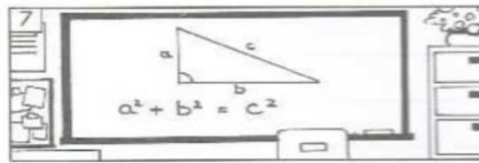
mathematics
